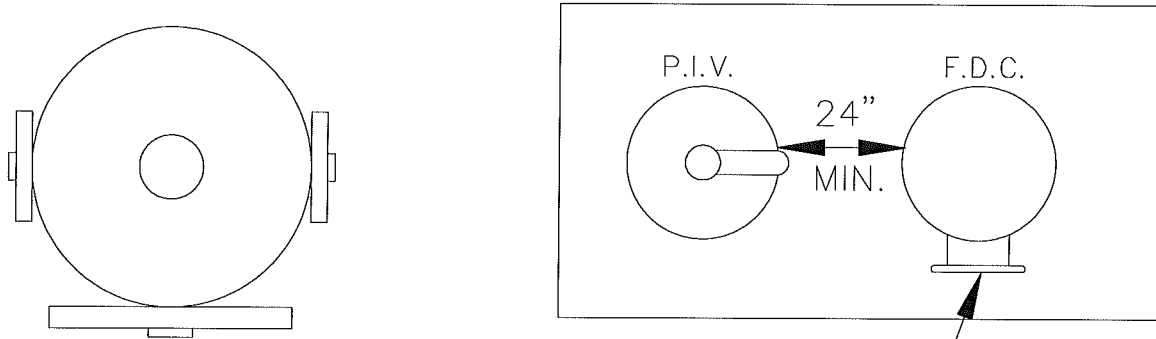
5" STORZ CONNECTION @ 30 DEG. ANGLE WITH CAP
